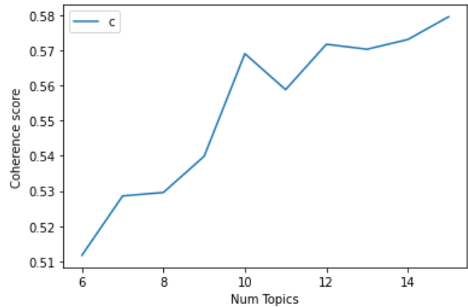
Fig. 2. Coherence score depending on the number of topics for the LDA model trained on comments
