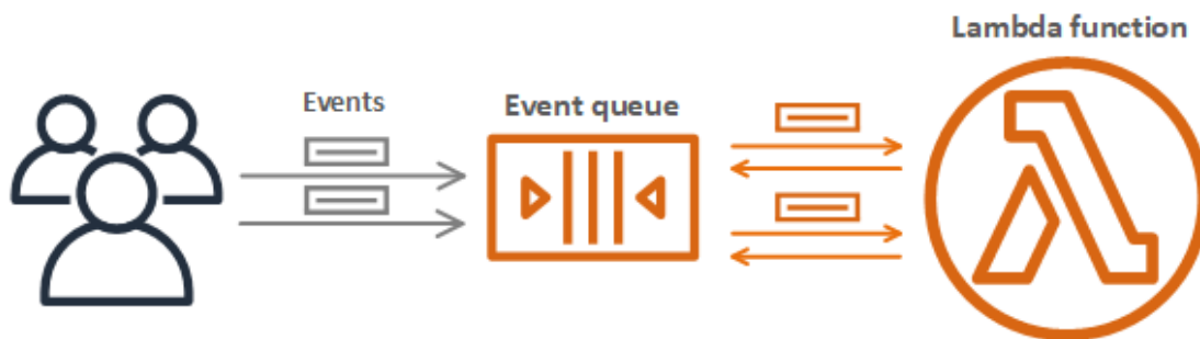
Image 8 - Asynchronous invocation overview [50]
